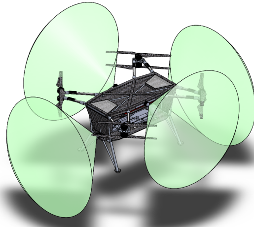
Figure 18: Detect and Avoid Sensor Coverage
